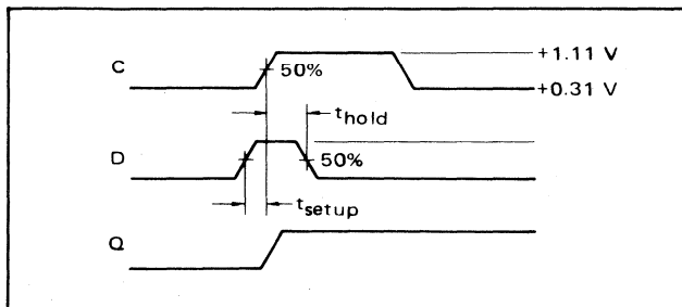
FIGURE 10 – Setup and hold time waveforms.
