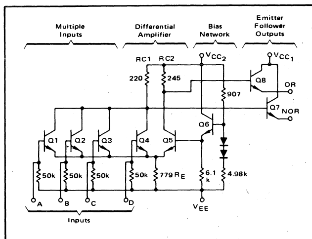
FIGURE 1 — Basic MECL 10,000 gate structure.
